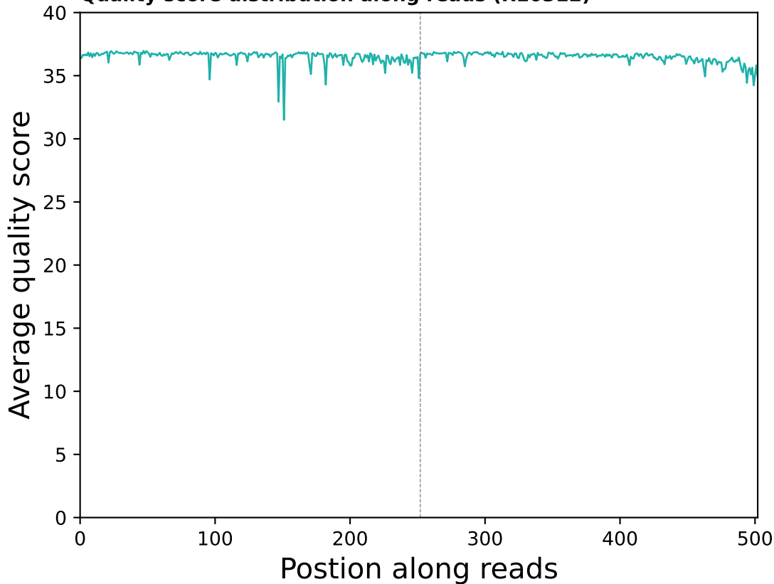
Quality score distribution along reads (R10312)
